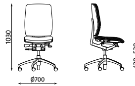
GLOBELINE COMFORT-6
