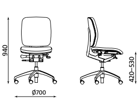
GLOBELINE-4
