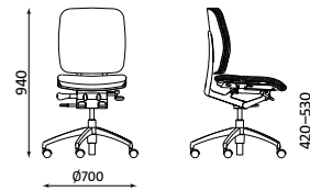
GLOBELINE COMFORT-4
