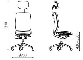
GLOBELINE-8
