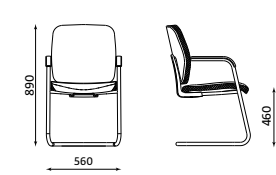
GLOBELINE COMFORT-5-A
